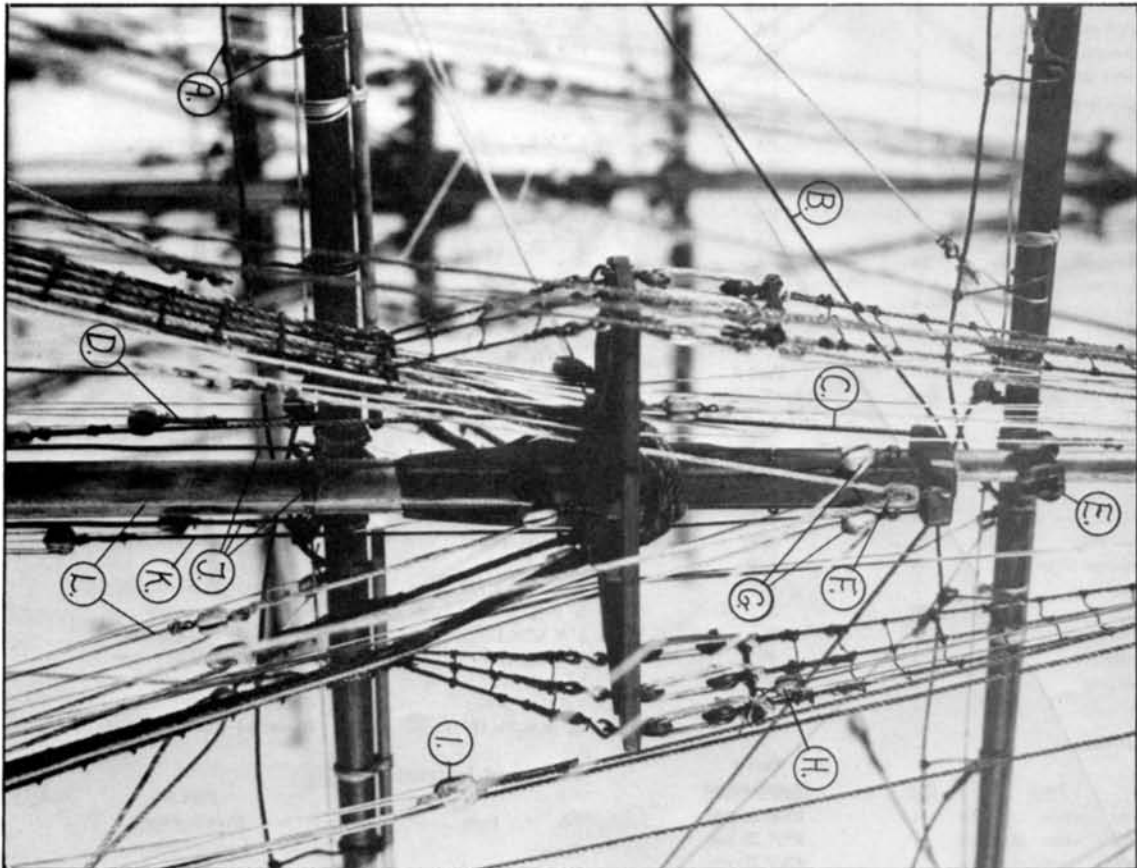
Main top, looking forward. A. Footropes and stirrups, B., C. Main lower yard lifts, D. Main topsail sheet, E. Main topsail yard parrels, F. Peak Halyard, G. Main boom topping lifts, H. Burton tackle, I. Main topsail halyard, J. Main lower yard truss, K. Main lower yard lifts, L. Throat halyard.
