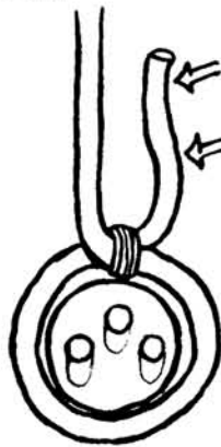
THROAT SEIZING
