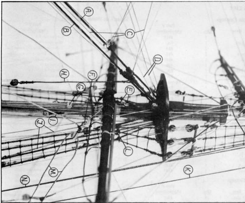
Main top. A. Main stay, B. Main preventer stay, C. Fore topsail braces, standing and running parts, D. Fore braces, standing and running parts, E. Main lower yard sling, F. Main clew garnet block, G. Main topsail sheet, H. Main stay tackle, I. Main tack, J. Main mast tackle runner, K. Main topgallant backstay, L. Futtock stave, M. Main sheet, N. Main topmast backstay.
