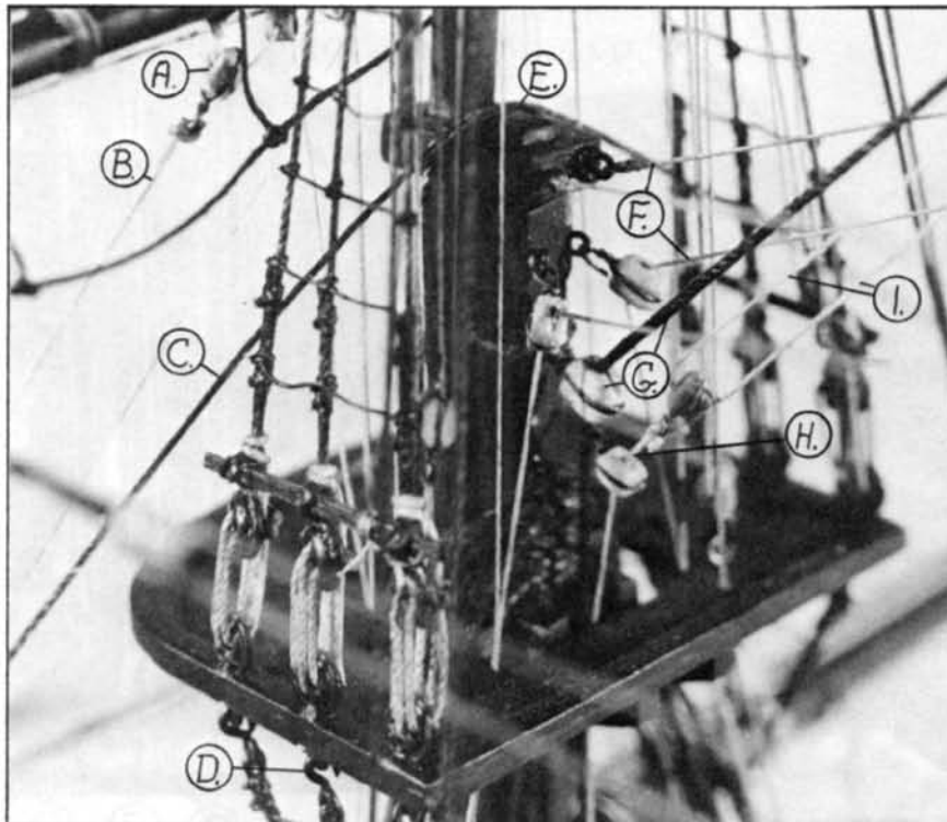
Fore top, looking forward. A. Fore topsail clewline block, B. Fore topsail sheet, C. Fore lower yard lift, D. Futtock hooks, E. Lower yard lifts, crossing over at cap, F. Main topsail braces, standing and running parts, G. Main topmast stay and fairlead block, H. Main topmast staysail downhaul, I. Main topmast staysail halyard.
