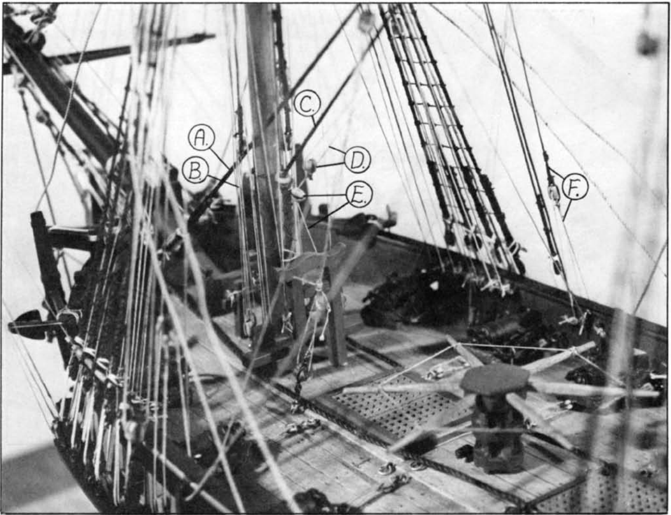
Main deck, looking forward. A. Main stay, B. Fore lower yard trusses. C. Main preventer stay, D. Main staysail halyard, E. Main staysail downhaul. F. Fore topgallant backstay and runner.
