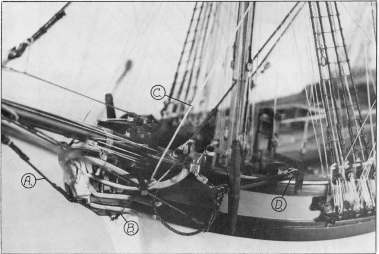
Port Bow. A. Bobstay, B. Fore tack boomkin guy, C. Fore tack, D. Anchor lashings.
