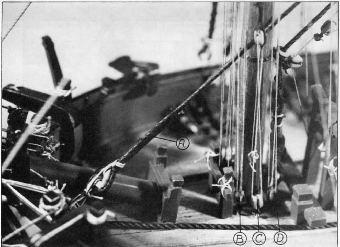
Port Bow. A. Bobstay, B. Fore tack boomkin guy, C. Fore tack, D. Anchor lashings.
